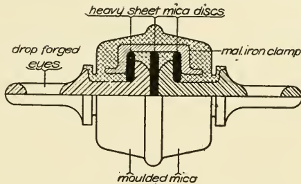
Fig. 190. Section of Strain Insulator
